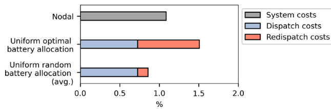
Fig. 4. Relative reduction of supply costs due to batteries in the nodal and uniform setting compared to the case without batteries (2030).
