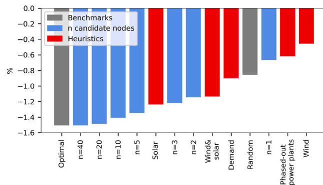
Fig. 6. Supply cost differences between different battery allocation scenarios and the uniform setting without batteries (2030).
