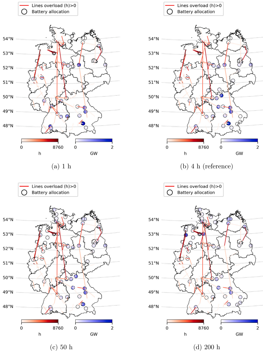
Fig. D.7. Optimal battery allocation based on the distribution of wind and solar in the uniform setting for different battery volume factors.
