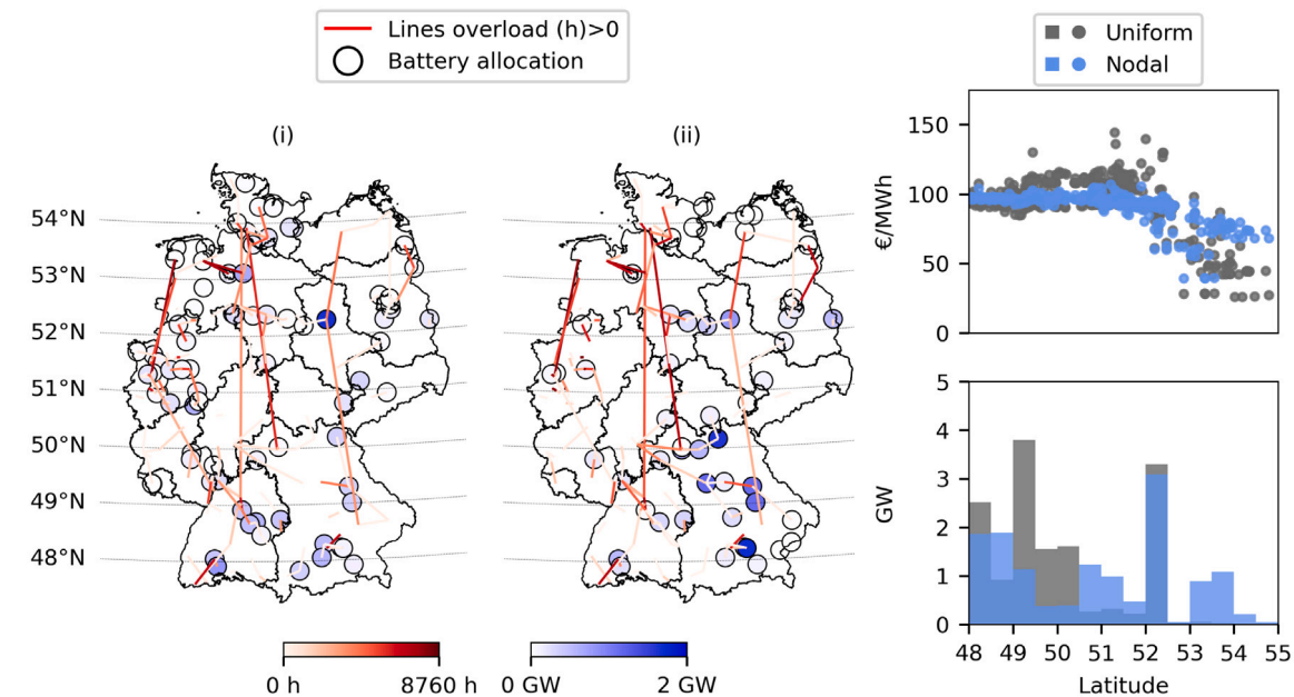
(a) Optimal allocation of battery capacity and line utilization in the (i) nodal and (ii) uniform setting
