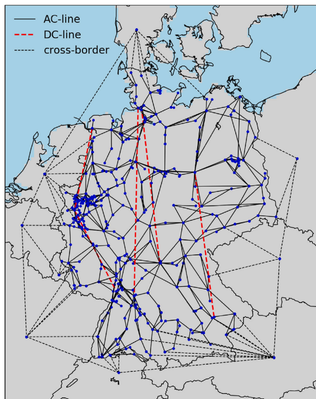
Fig. 2. German transmission grid and NTC connections to neighboring countries.
