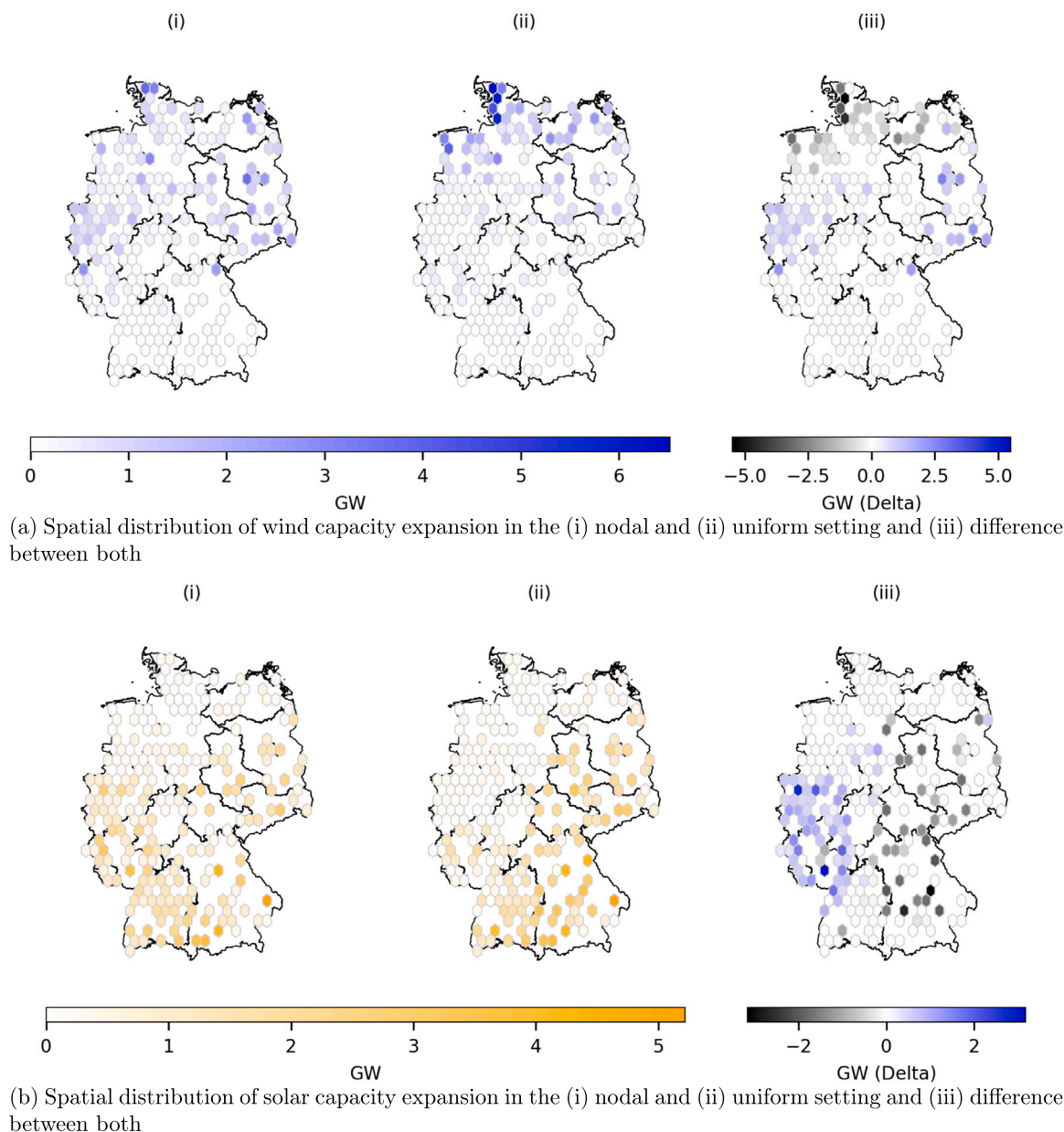
Fig. 3. Spatial distribution of wind and solar capacity expansion in the nodal and uniform setting (2030)
