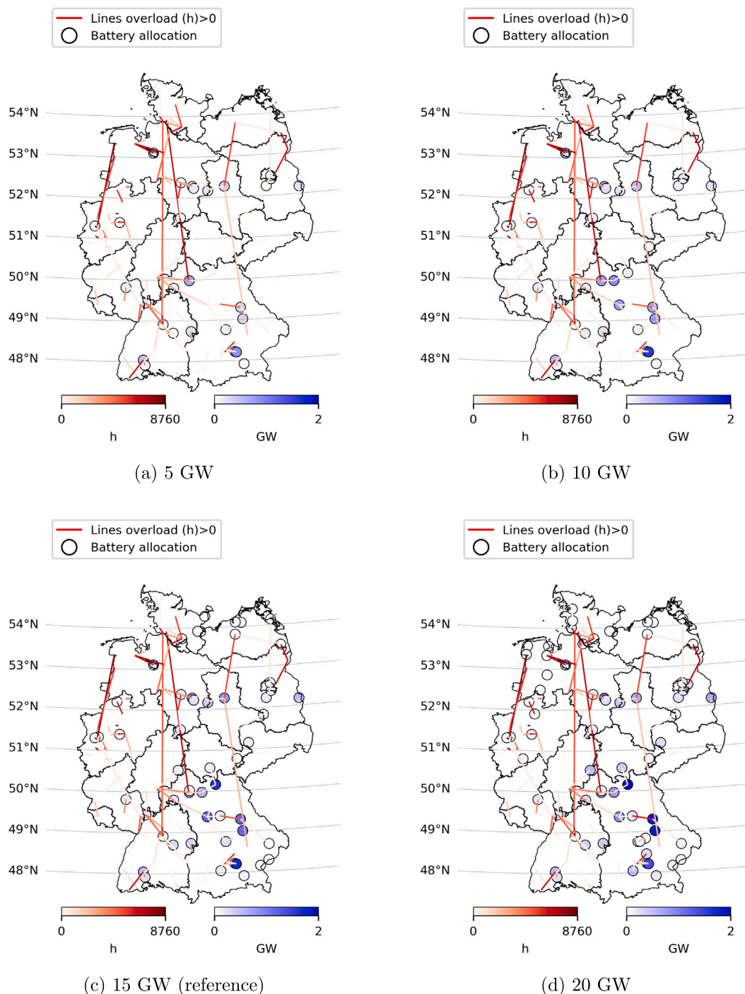
Fig. D.8. Optimal battery allocation based on the distribution of wind and solar in the uniform setting for different battery capacities.
