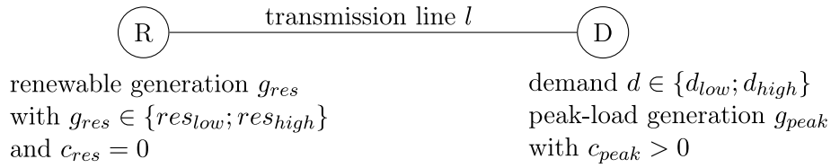
Fig. 1. Two-node example.
