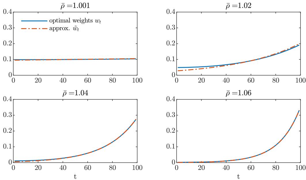
FIGURE 2 | Approximation to optimal weights for different values of \bar{\rho} . The optimal weights w_t are obtained as the eigenvector corresponding to the largest eigenvalue of \Psi_{\bar{\rho}} . Approximate optimal weights as in Equation (10).
