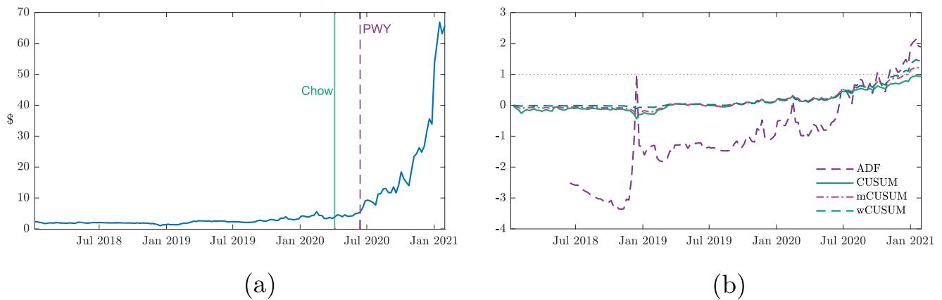
FIGURE 6 | Results for plug power. (a) Price of plug power and bubble dates, (b) sequence of normalized bubble detectors.
