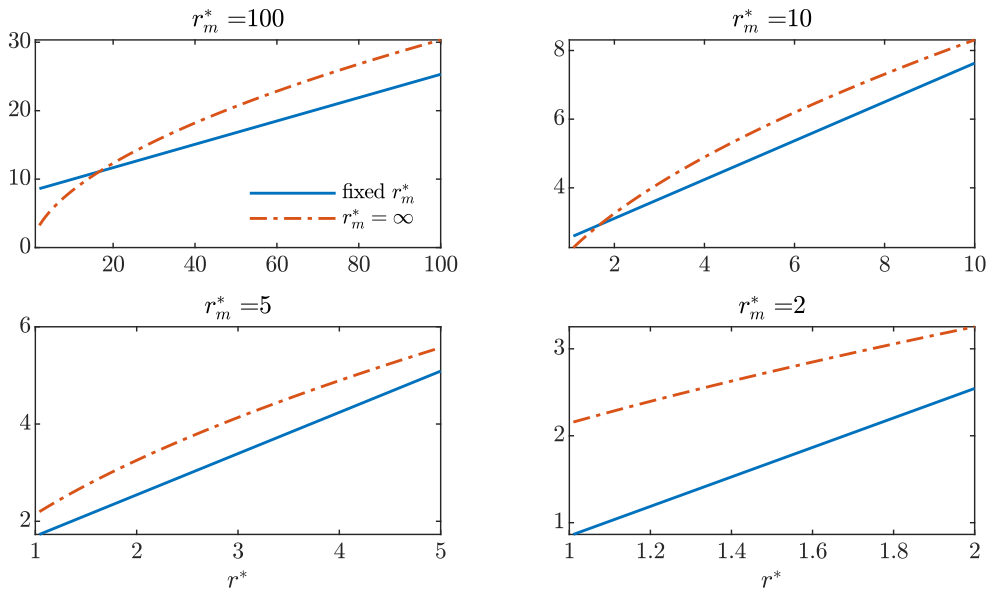
FIGURE 3 | CUSUM boundary functions for infinite vs. fixed horizon monitoring. x-axis is normalized by the relative time index r^* = t/T_0 , where T_0 is the number of training sample periods. Hence, r^* > 1 refers to the monitoring sample.
