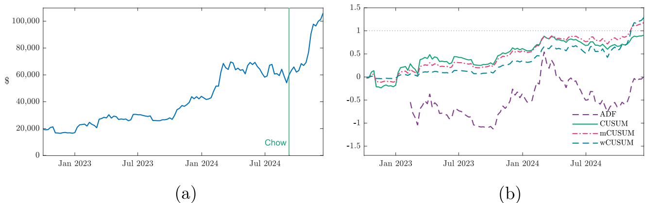
FIGURE 7 | Results for Bitcoin. (a) Price of Bitcoin and bubble dates, (b) sequence of normalized bubble detectors.
