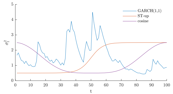
FIGURE 4 | Different variance profiles.
