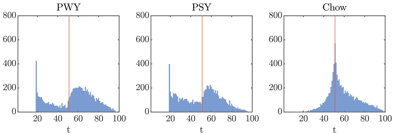
FIGURE 5 | Distribution of date-stamping estimators. Histograms from date-stamping estimates based on 10,000 MC repetitions with T = 100 . The vertical line at observation t = 51 indicates the true emergence of the bubble.
