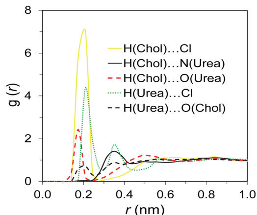
Fig. 4 Atom-atom RDFs between DES components in the pure system.
