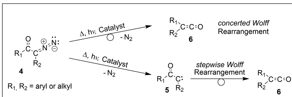
Scheme 2 The Wolff rearrangement reaction of \alpha -diazo ketone 4 leads to the \text{N}_2 loss upon activation, generating \alpha -keto carbene intermediate 5 with an electron sextet at the carbon atom, ultimately delivering ketenes 6 in a stepwise rearrangement reaction or along a direct concerted reaction pathway. 5,6
