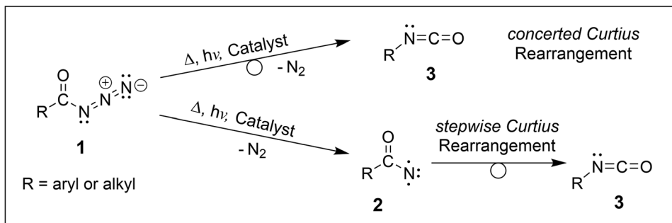
Scheme 1 The Curtius rearrangement reaction of acyl azides 1 leads to the \text{N}_2 release upon activation and ultimately yields isocyanates 3 either via acyl nitrene intermediates 2 (shown here in the triplet electronic state with two unpaired electrons) in a stepwise reaction or along a direct concerted reaction pathway. 3
