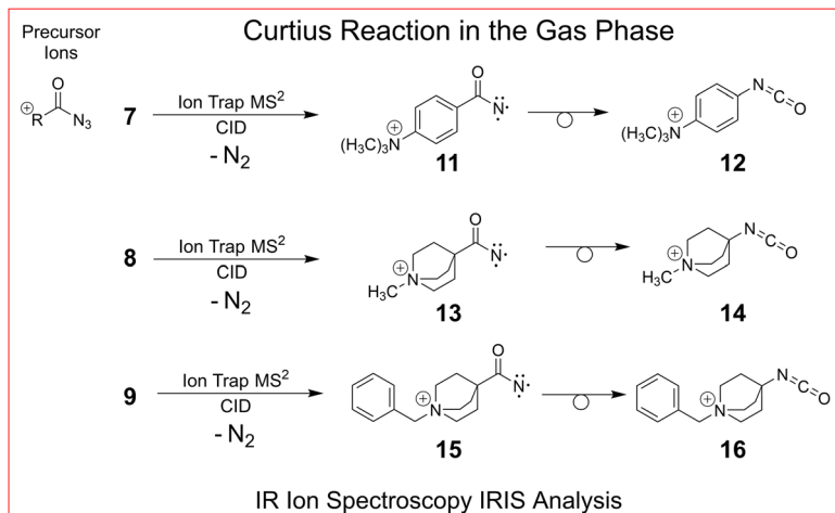
Scheme 4 The three remotely charge-tagged acyl azide molecular ions 7–9 produced by (+)ESI-MS are collisionally activated in the gas phase of a quadrupole ion trap (see Fig. 3 and Fig. S24 and S26 in the ESI†; gas-phase chemistry in the red box). The nature of the product ions, i.e. , nitrenes or isocyanates, generated upon CID (potential product ions 11 or 12 of 7 , 13 or 14 of 8 , and 15 or 16 of 9 ), as well as the molecular structures of the acyl azide precursors 7–9 are investigated in the gas phase via IRIS.
