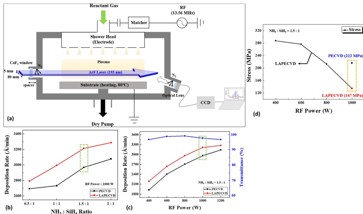
Fig. 5 (a) Schematic of the LAPECVD system; deposition rates for PECVD and LAPECVD, measured as functions of \text{NH}_3 : \text{SiH}_4 ratio (b) and RF plasma power (c); and (d) residual stress of silicon nitride films with plasma RF power, reused with permission from Elsevier. 152
