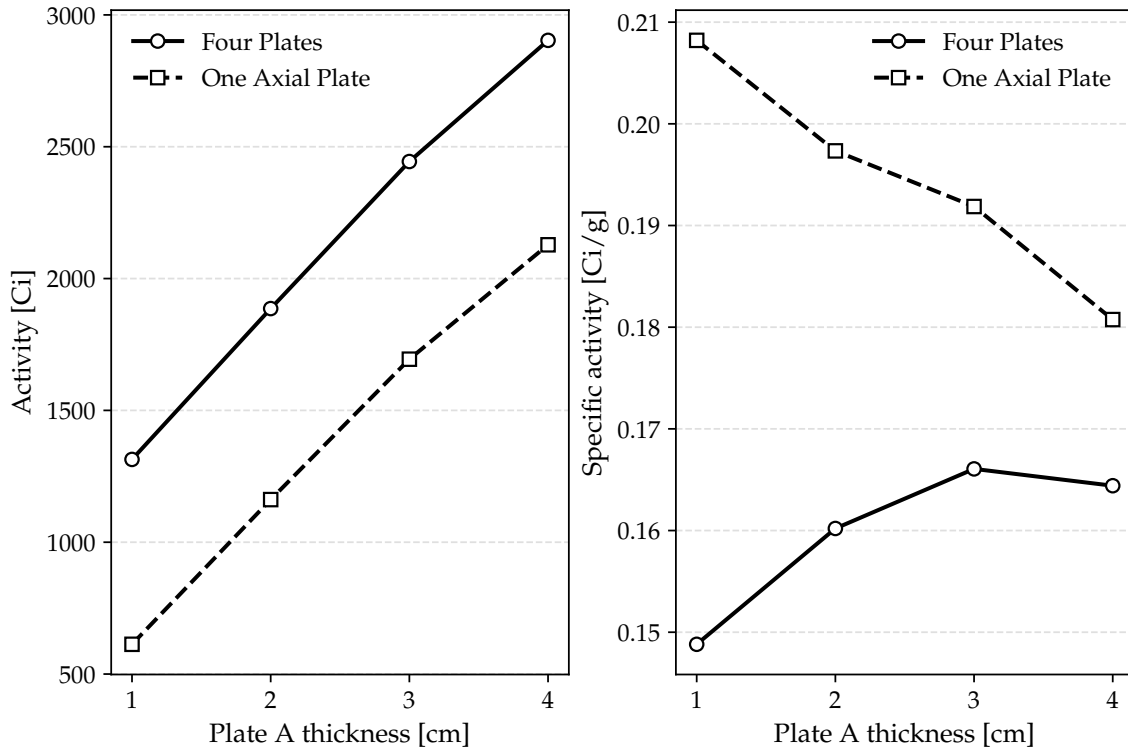
Figure 5.8: ^{99}\text{Mo} activity and specific activity for the \text{MgO-H}_2\text{O} system as a function of axial plate (Plate A) thickness after 6 days of irradiation.
