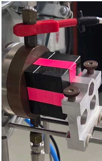
(a) Experimental irradiation setup at the INM-5 accelerator facility.
