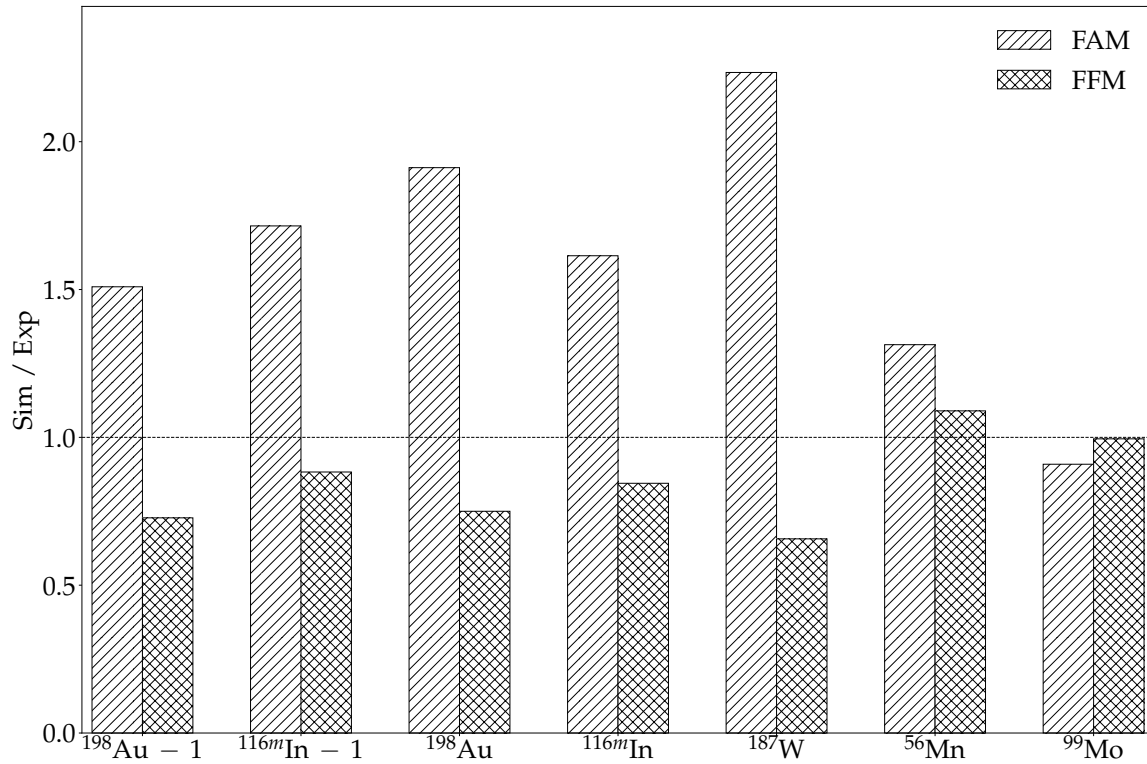
Figure 4.11: Ratios of simulated to experimentally measured activities for Cd-covered foil irradiation.
