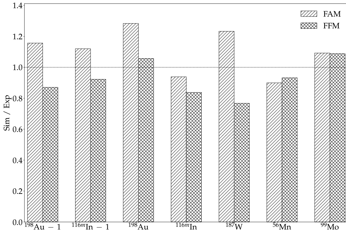
Figure 4.9: Ratios of simulated to experimentally measured activities for bare foil irradiations.
