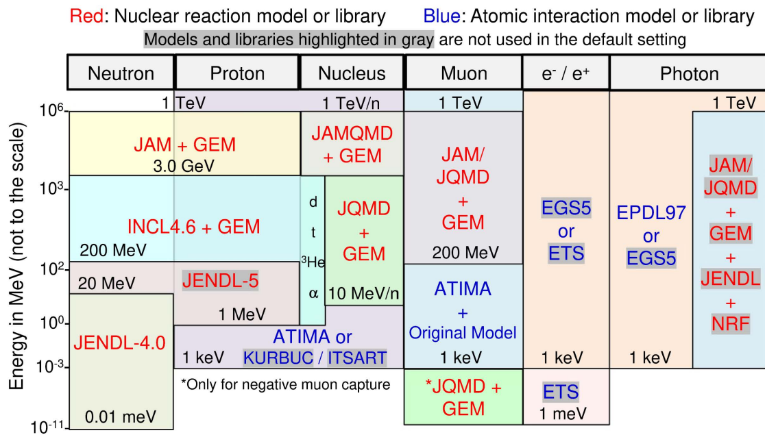
Figure 3.1: Recommended physics models and data libraries for use in PHITS obtained from [29].
