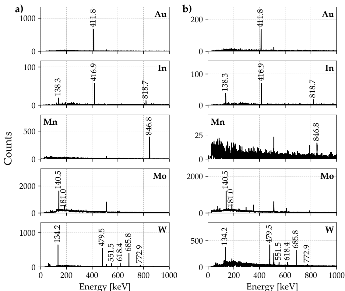
Figure 4.5: Representative \gamma -ray spectra obtained for selected activation foils in the extended multiple-monitor study for a) bare foil irradiation and b) Cd-covered irradiation.
