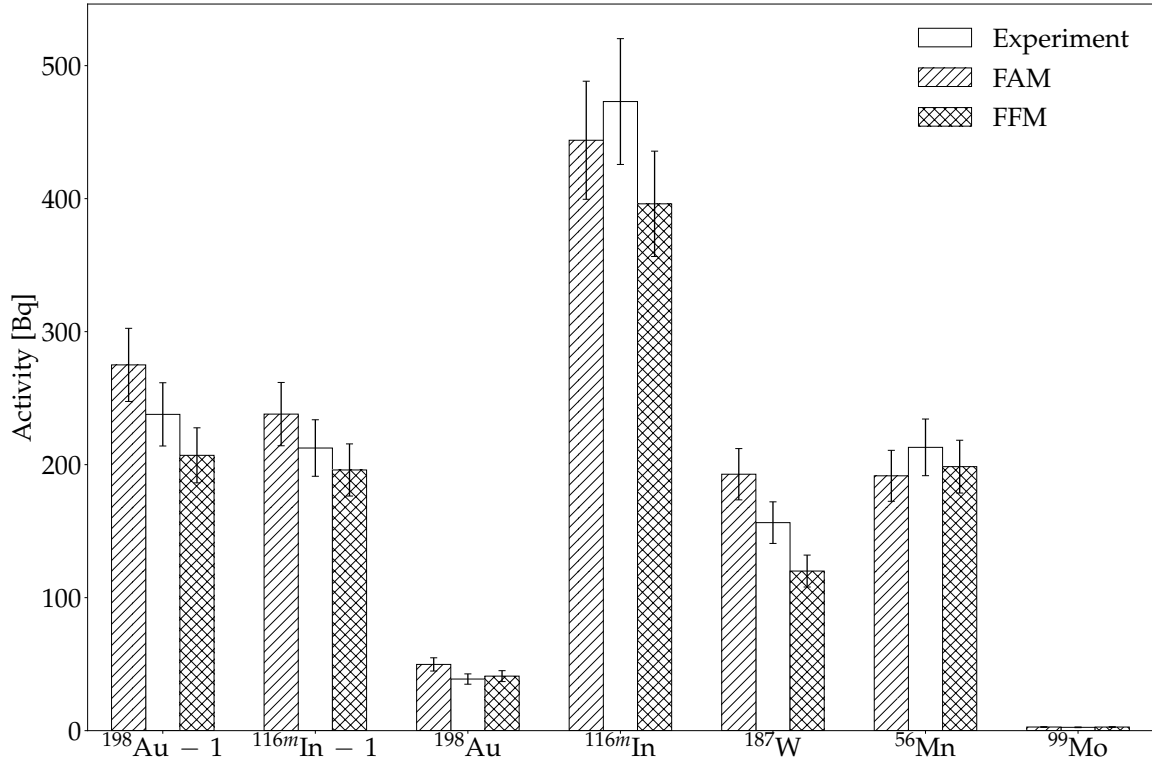
Figure 4.8: Experimental and simulated activities at the EOI for the bare foils.
