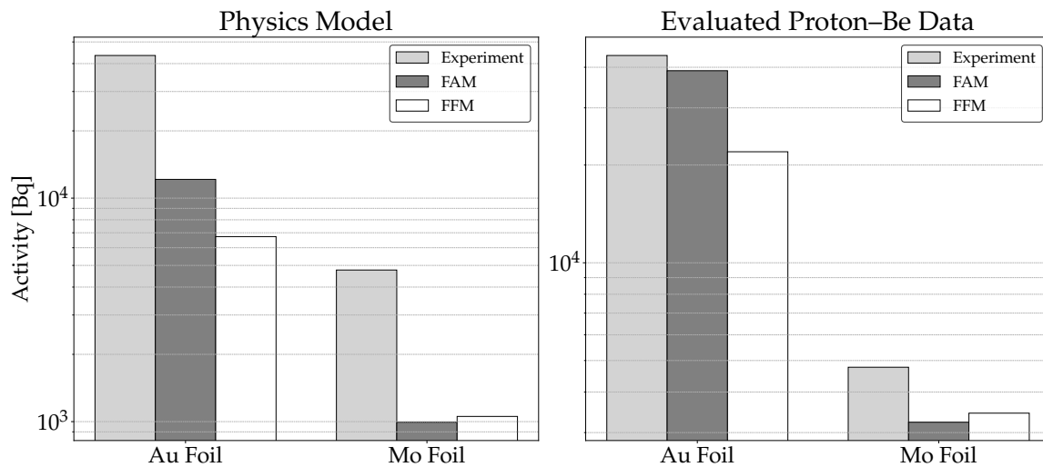
Figure 5.13: Comparison of experimentally measured activation foil activities with activities predicted using the FAM and FFM. The left panel shows results obtained using the default PHITS proton-induced reaction models for neutron production in Be, whereas the right panel shows results obtained using evaluated nuclear data.
