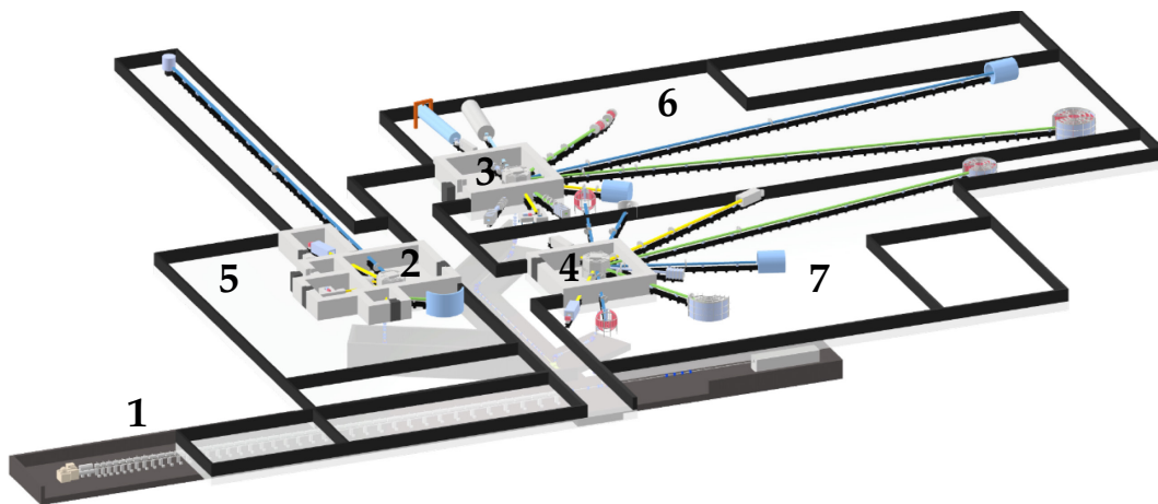
Figure 1.6: Overview of the High Brilliance neutron Source (HBS) concept including the linear accelerator system (1), target-moderator-reflector (TMR) assemblies (2, 3, 4), and representative instrument halls (5, 6, 7). The schematic illustrates the accelerator-driven neutron production concept and the extraction of neutron beams to multiple instrument stations.
