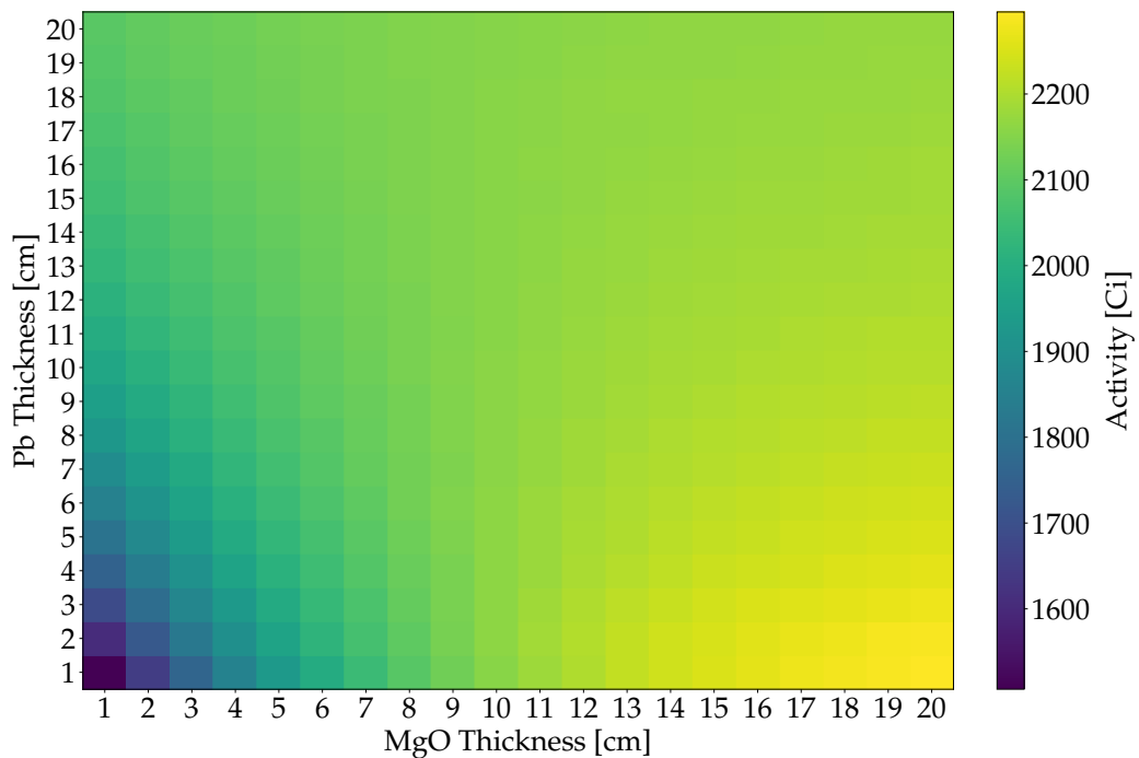
Figure 5.10: Calculated total ^{99}\text{Mo} activity for composite reflector configurations consisting of an inner MgO layer and an outer Pb layer, shown as a function of the MgO and Pb thickness. The activity corresponds to the sum over the investigated irradiation regions.
