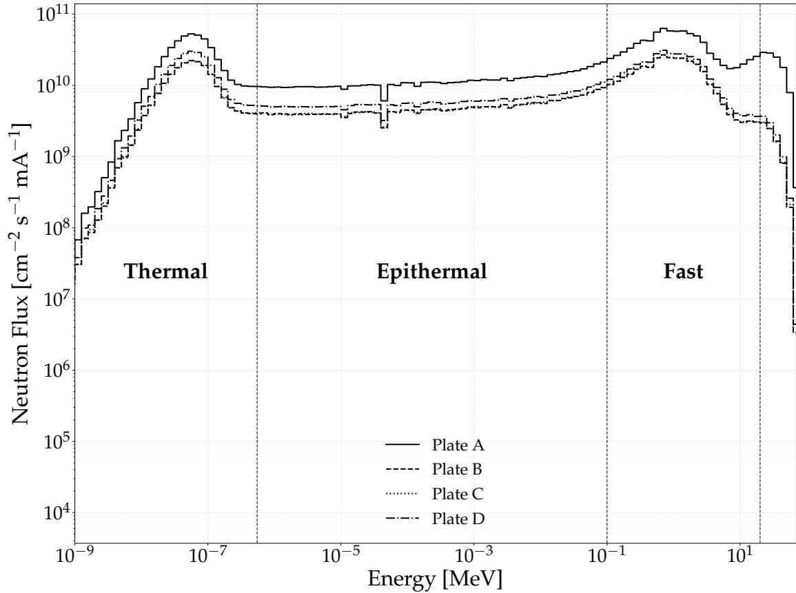
Figure 5.5: Simulated neutron energy spectra within the Mo plates positioned at a distance of 3 cm from the Al casing, with a 5 cm \text{H}_2\text{O} moderator and 10 cm Pb reflector.
