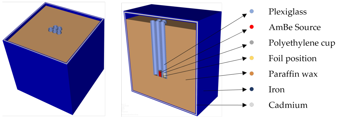
Figure 4.1: Geometrical model of the irradiation facility used for the neutron activation experiments and corresponding simulations. The figure shows a top view of the paraffin moderator with the embedded plexiglass tubes and a vertical cross-section along the symmetry axis of the central tube containing the AmBe neutron source and surrounding materials.
