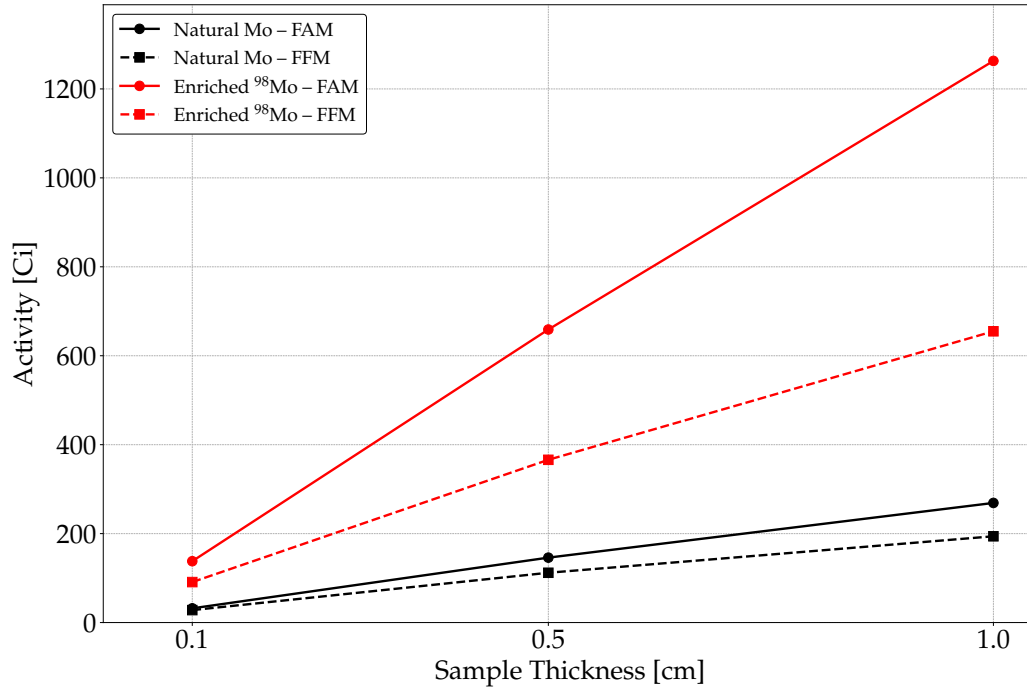
Figure 5.9: Comparison of ^{99}\text{Mo} activities calculated using the FAM and FFM for natural and enriched ^{98}\text{Mo} targets as a function of target thickness. Results are shown for a 12 \times 12 \text{ cm}^2 irradiation plate positioned 1.35 cm from the target.
