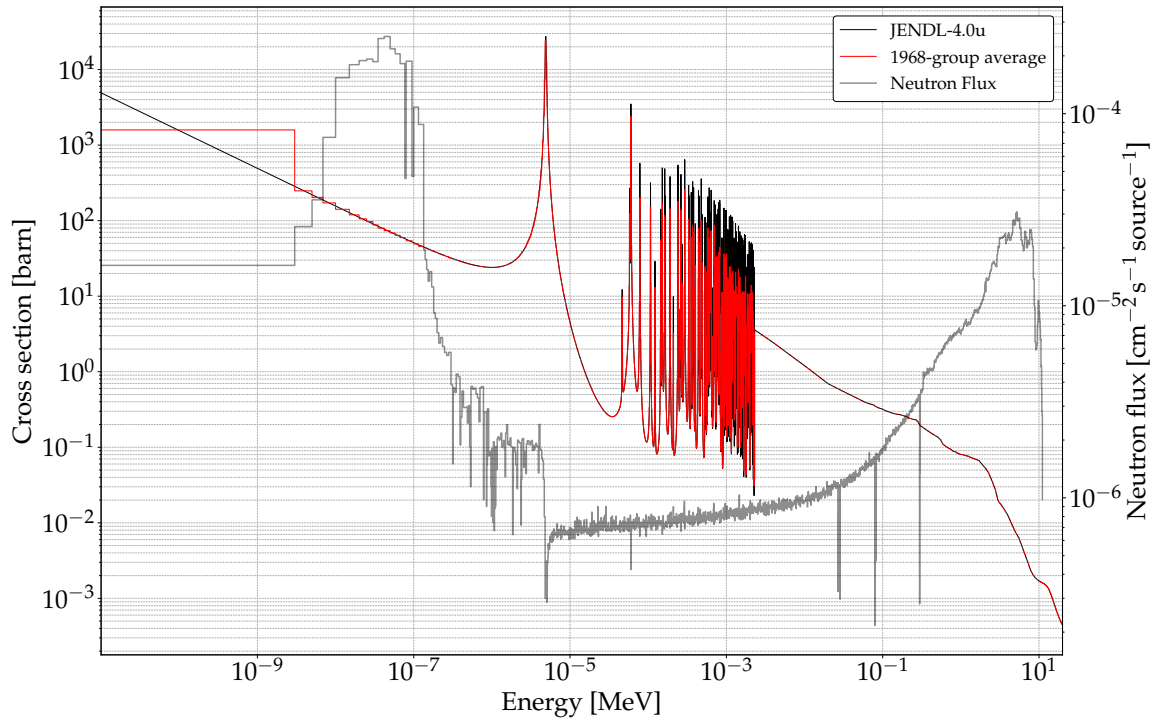
Figure 3.5: Illustration of the flux folding procedure. The energy-dependent neutron capture cross section for ^{197}\text{Au}(n,\gamma)^{198}\text{Au} reaction, its multi-group representation, and the corresponding neutron flux spectrum within the gold foil with a thickness of 0.0025 cm are shown. The reaction rate is obtained by folding the flux with the cross section over all energy groups.
