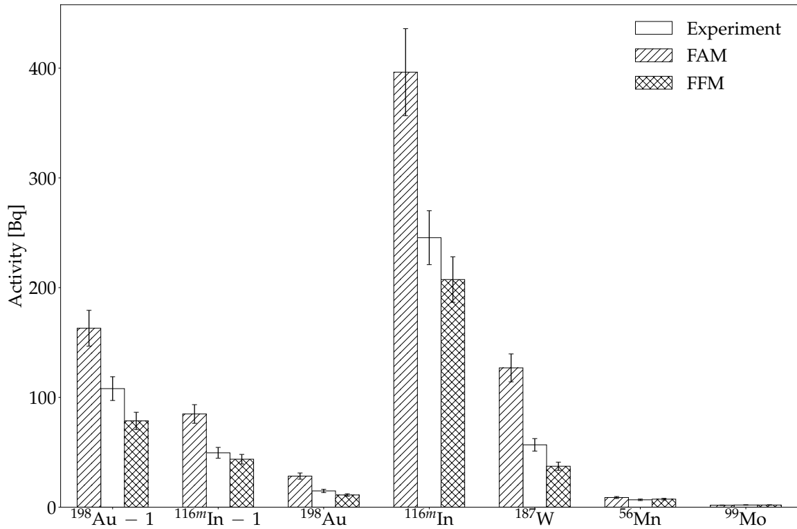
Figure 4.10: Experimental and simulated activities at the end of irradiation for Cd-covered foils.
