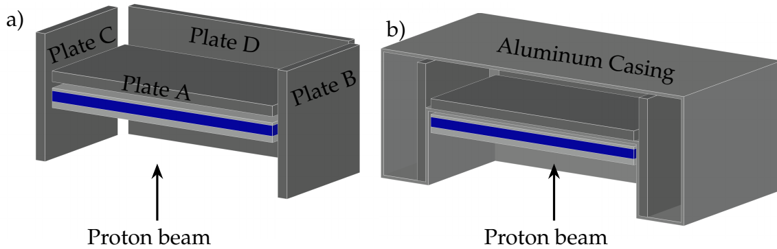
Figure 5.3: Geometric model of the (a) arrangement of the four irradiation plates (A–D) around the Ta target and (b) aluminum casing (Al casing) enclosing the assembly and defining the moderator volume.
