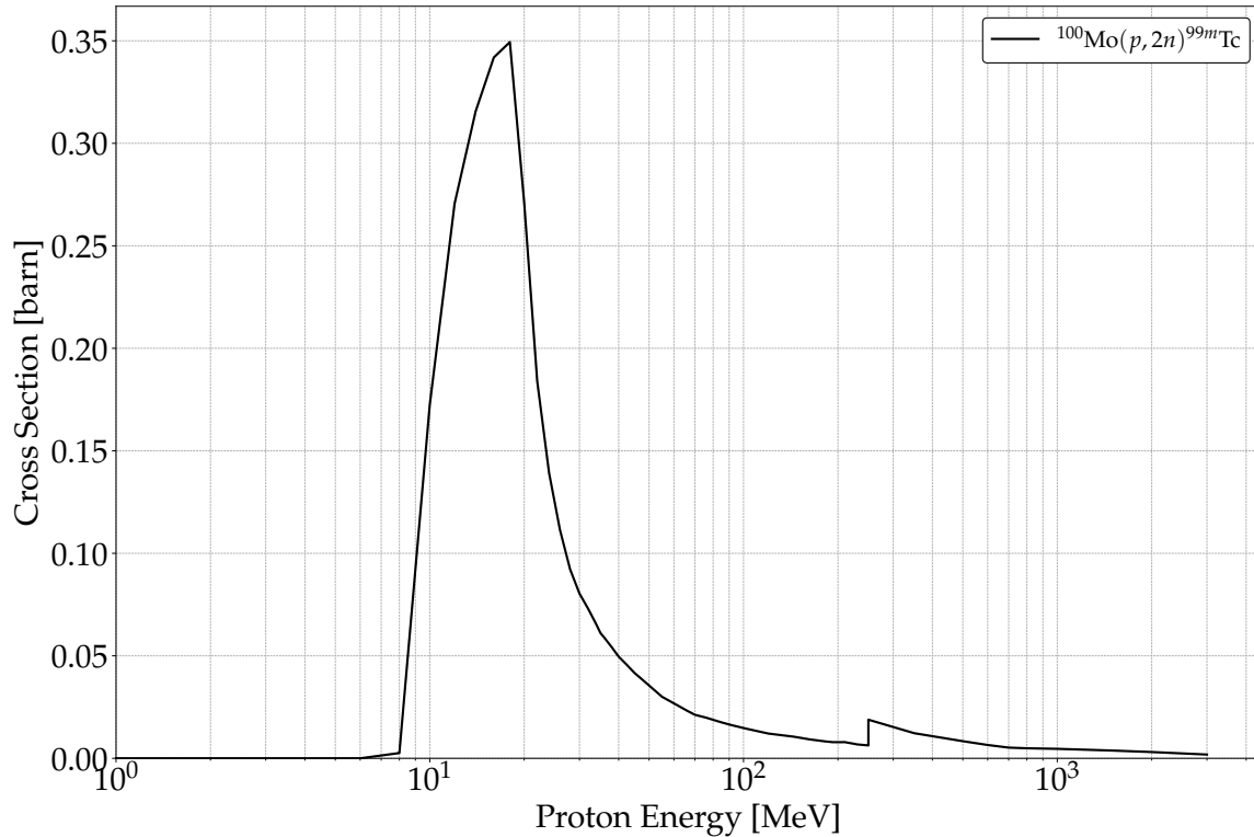
Figure 1.3: Representative excitation function of the ^{100}\text{Mo}(p, 2n)^{99m}\text{Tc} reaction from the TENDL evaluated nuclear data library [22], accessed through JANIS Web [20] illustrating the dependence of reaction cross section on proton energy. The optimal production window is typically located between approximately 16 and 24 MeV.
