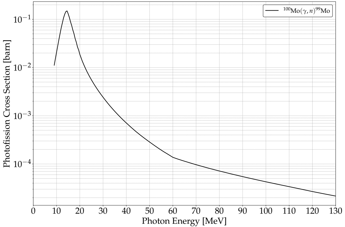
Figure 1.5: Representative cross section of the ^{100}\text{Mo}(\gamma, n)^{99}\text{Mo} reaction from the ENDF/B-VIII.1 evaluated data library [23], accessed through JANIS Web [20], as a function of photon energy showing the giant dipole resonance region relevant for photonuclear production.
