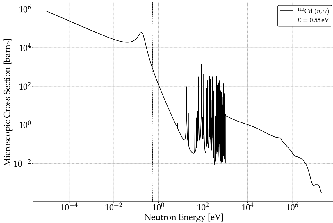
Figure 2.2: Microscopic neutron capture cross section of ^{113}\text{Cd} from the ENDF/B-VIII.1 evaluated data library [23], accessed through JANIS Web [20], as a function of neutron energy.
