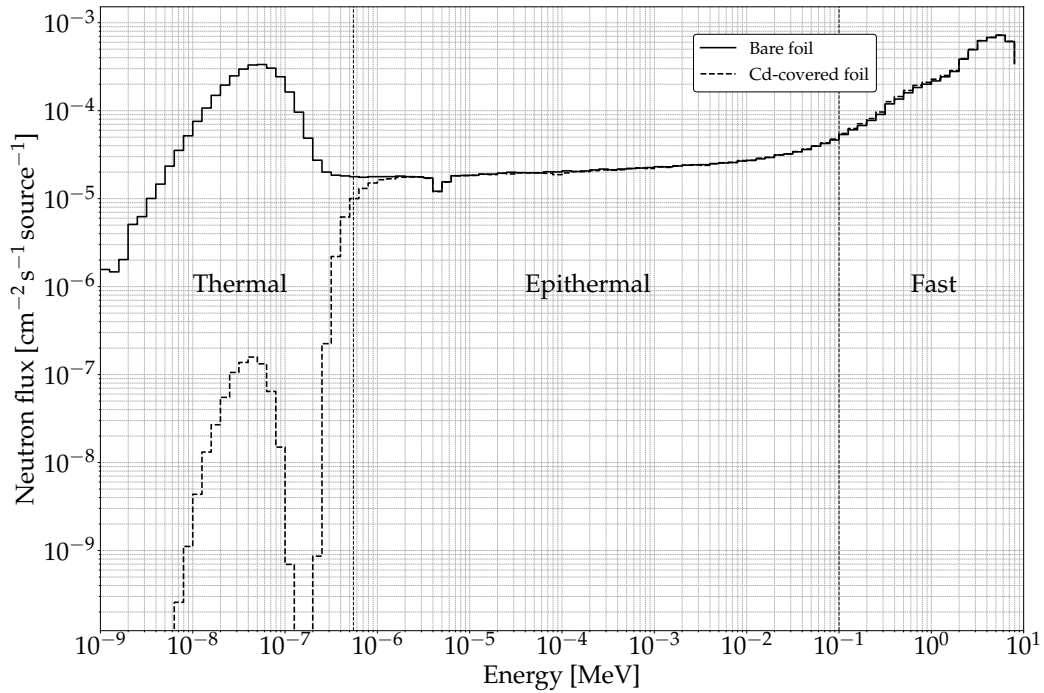
Figure 4.4: Simulated neutron energy spectrum within the Au – 1 foil for bare and Cd-covered irradiations.
