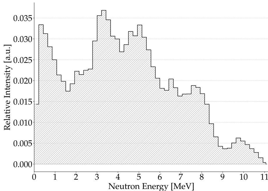
Figure 4.3: AmBe neutron energy spectrum used in this work. [57]
