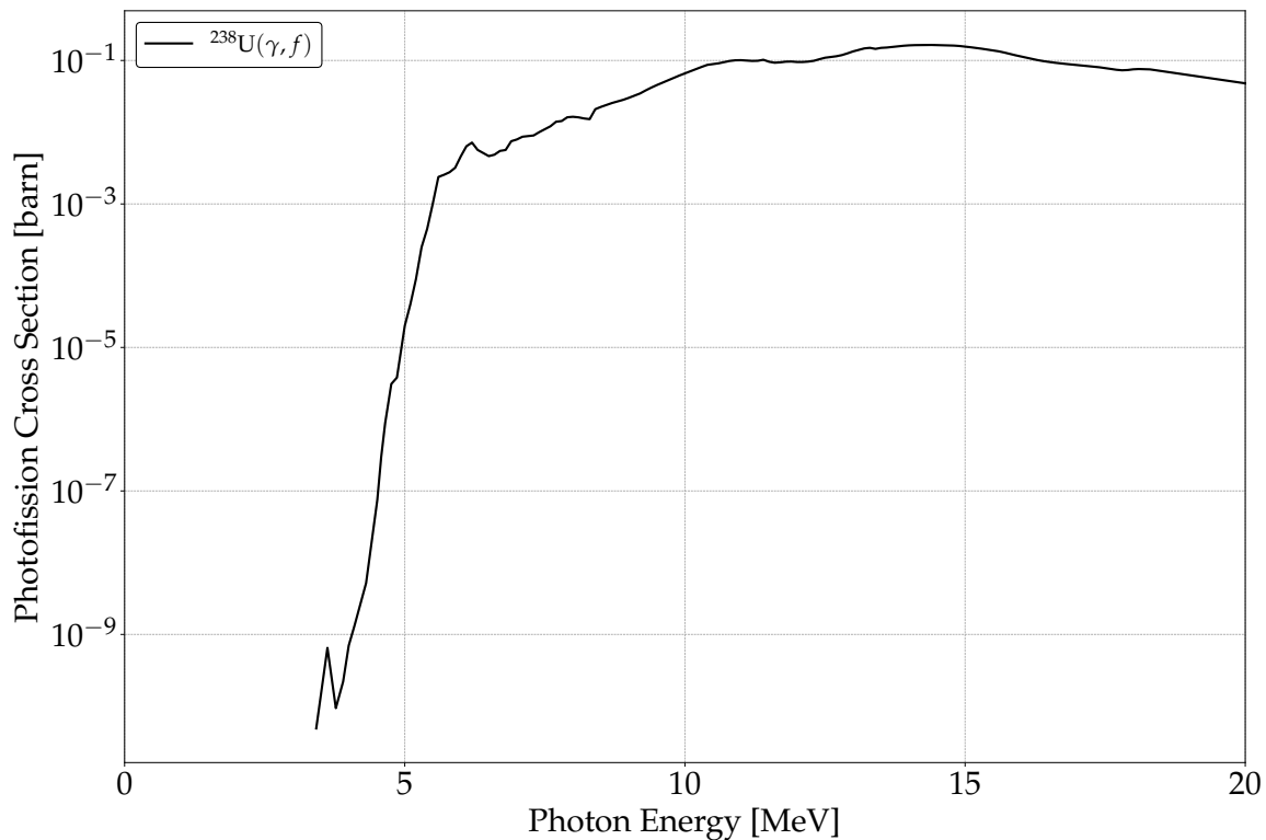
Figure 1.4: Representative photo-fission cross section of ^{238}\text{U} from the ENDF/B-VIII.1 evaluated nuclear data library [23], accessed through JANIS Web [20], as a function of photon energy.
