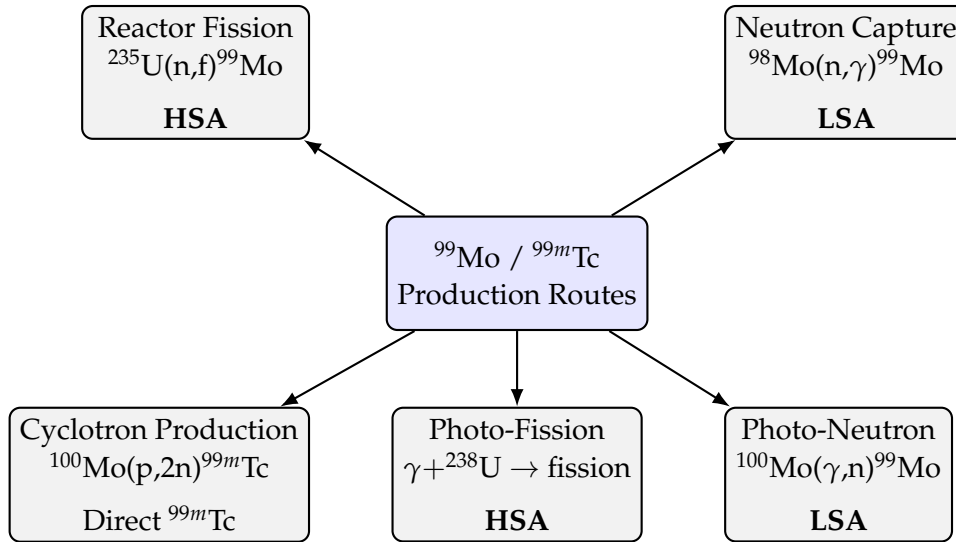
Figure 1.1: Overview of principal ^{99}\text{Mo} and ^{99m}\text{Tc} production routes and their corresponding specific activity classifications. HSA: high specific activity and LSA: low specific activity classifications refer to production routes where applicable.
