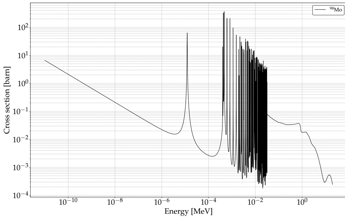
Figure 1.2: Energy-dependent neutron-capture cross section data for the ^{98}\text{Mo}(n, \gamma)^{99}\text{Mo} reaction from the JENDL-4.0 evaluated nuclear data library [19], accessed through JANIS Web [20].
