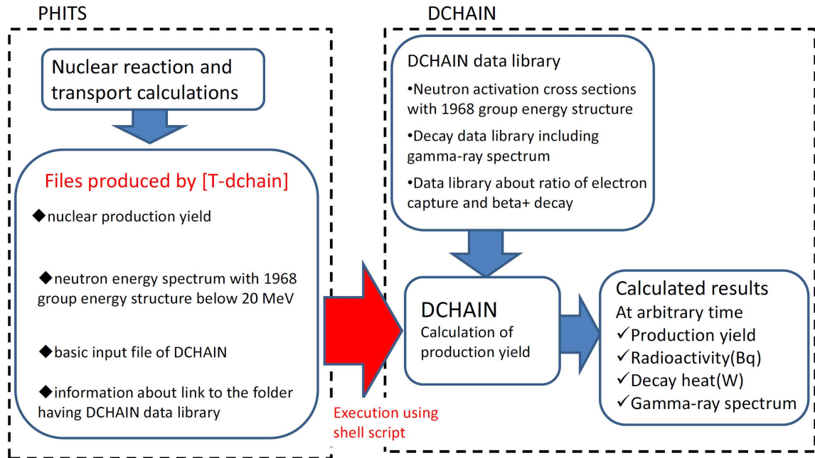
Figure 3.2: Concept of the coupled PHITS–DCHAIN calculation workflow obtained from [35].
