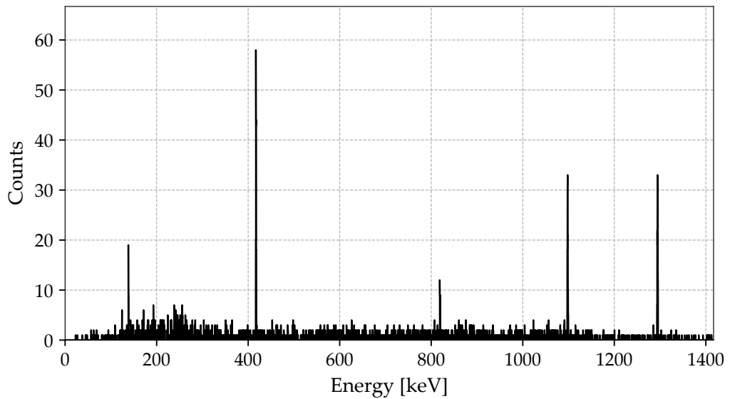
Figure 4.7: Enlarged bare-foil \gamma -ray spectrum for the ^{116m}\text{In} isotope used for activity determination.
