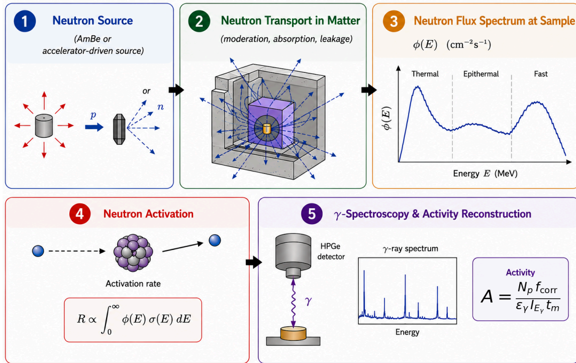
Figure 2.1: Simplified workflow linking neutron generation to experimentally reconstructed activities. (Layout drafted with AI-assisted graphics tools and finalized by the author.)
