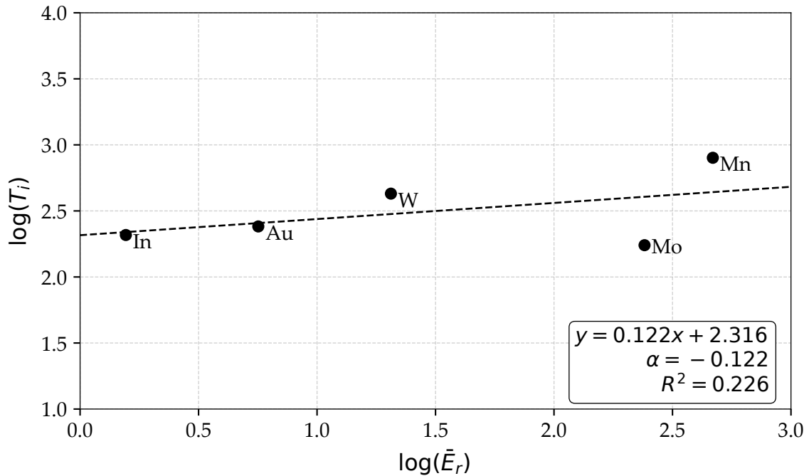
Figure 4.12: Representative determination of the epithermal shape factor \alpha using the Cd-covered multi-monitor k_0 -factors method. The value of \alpha is obtained from the slope of the fitted linear regression.
