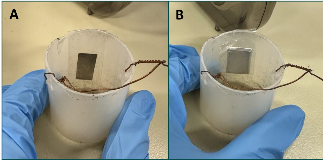
Figure 4.2: Polyethylene holder with (A) bare W sample and (B) Cd-covered W sample.
