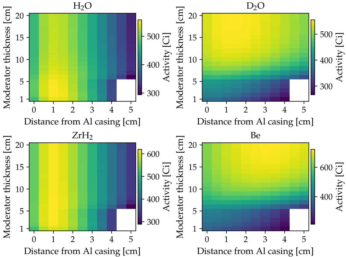
Figure 5.6: Calculated ^{99}\text{Mo} activity in Plate A for various moderators as a function of plate distance from the Al casing and moderator thickness, with a 5 cm Pb reflector.
