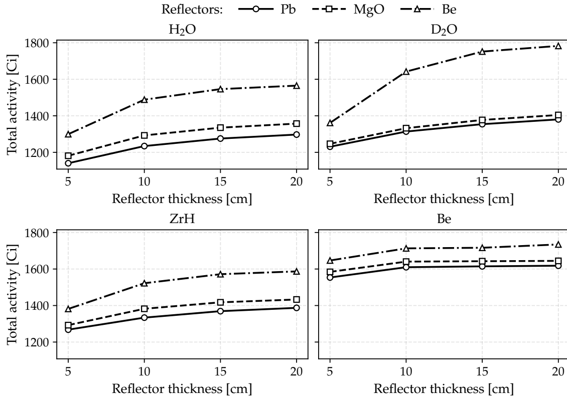
Figure 5.7: Total ^{99}\text{Mo} activity from all plates after 6 days of irradiation as a function of reflector thickness for different reflector materials (Pb, MgO, Be), shown separately for each moderator ( \text{H}_2\text{O} , \text{D}_2\text{O} , \text{ZrH}_2 , Be). For each moderator—reflector thickness combination, the plate distance and moderator thickness correspond to the highest activity configuration identified in the preceding analysis.
