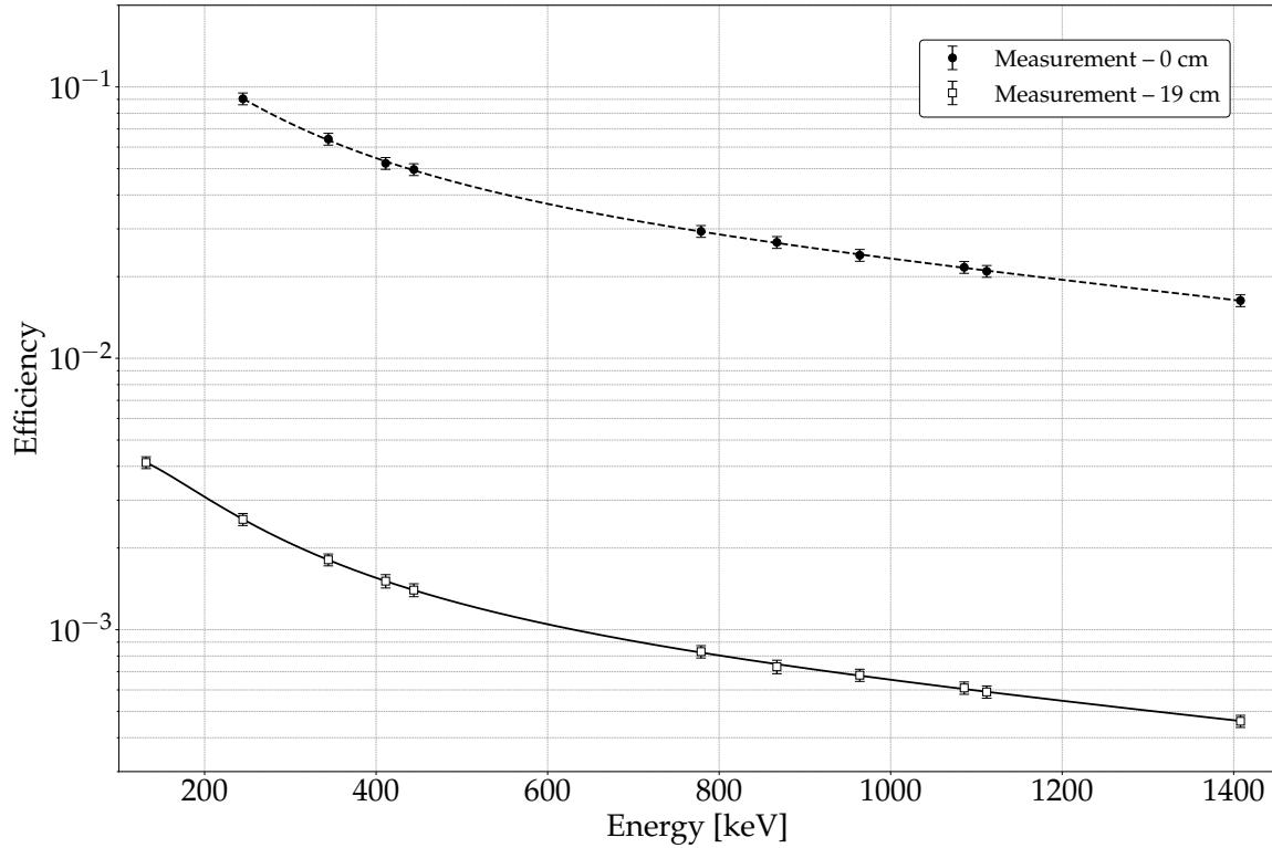
Figure 3.4: Energy dependence of the FEP efficiency for the two counting geometries. The lines represent the fit of the data with Eq. 3.2.
