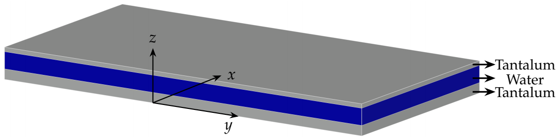
Figure 5.2: Geometrical model of the layered Ta–water–Ta target used in the simulations. The target has a surface area of 12 \times 24 \text{ cm}^2 and consists of a 0.6 cm Ta layer, a 1.0 cm water layer, and a 0.25 cm Ta back layer, for a total thickness of 1.85 cm.
