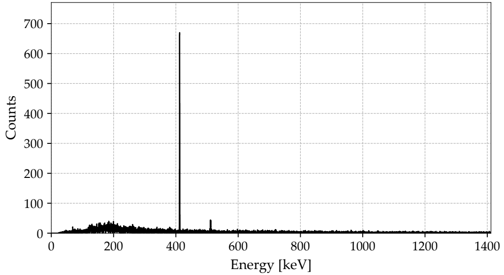
Figure 4.6: Enlarged bare-foil \gamma -ray spectrum for the ^{198}\text{Au} isotope used for activity determination.
