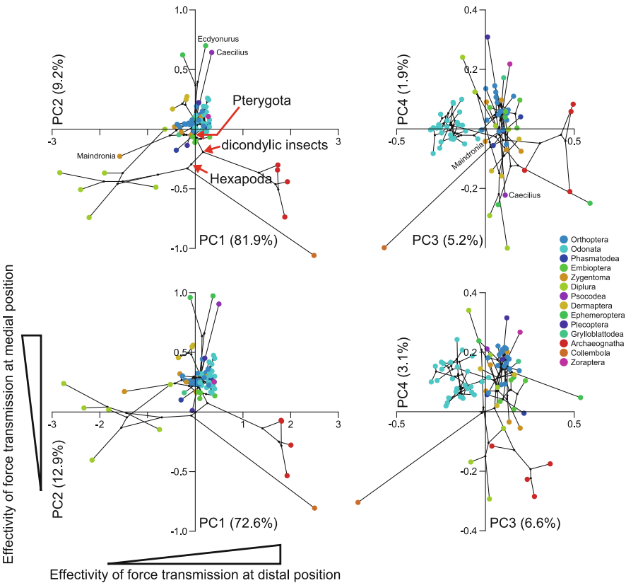
Fig. 6.5 Principal component analysis (PCA) of MA progression with the first four PCs shown. 2D plots of the first four uncorrected (upper row) and phylogeny-corrected PCs (lower row). Same lineage-specific color code as in Fig. 6.4. Note that the indication of the functional interpretation of the PCs in the lower left plot is also applicable to the upper left plot. Functional interpretations for PCs3+4 are not shown due to the low variance associated with these PCs
