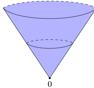
Figure 3.1: The Lorentz cone \mathcal{L}^3 .
