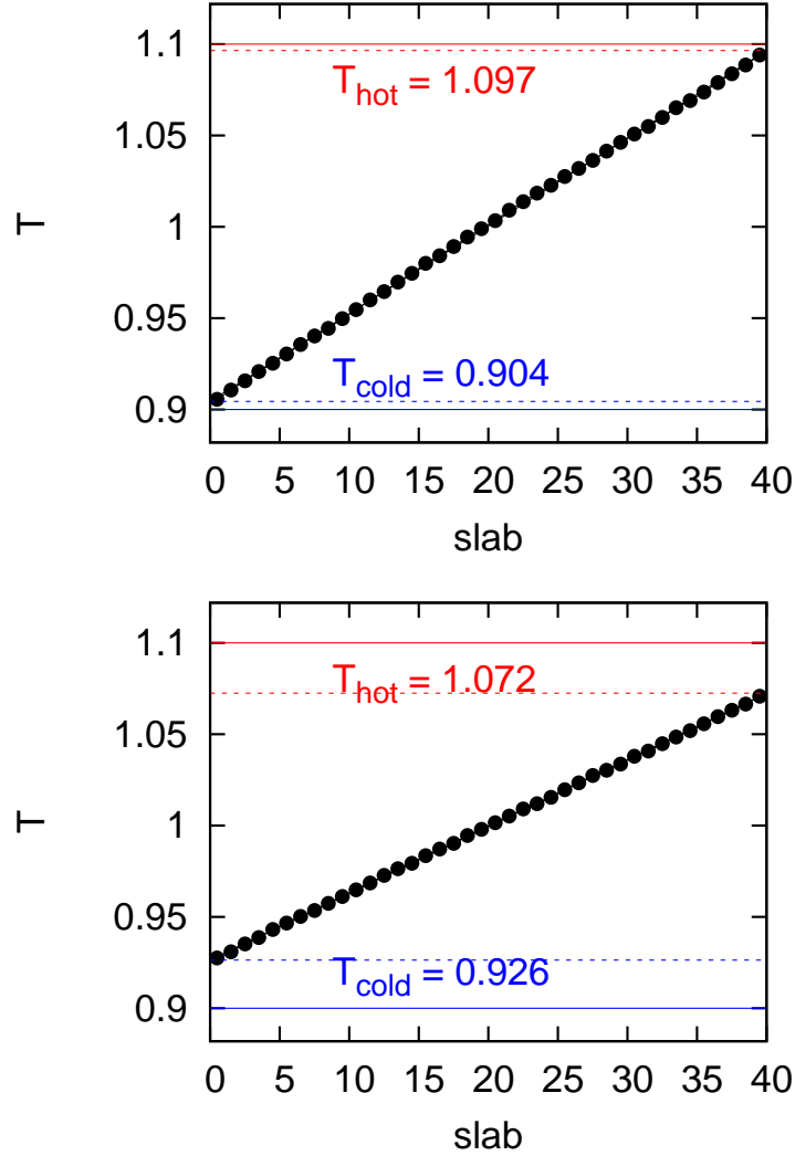
Figure 3.3: Temperature profiles of the MPC in contact with walls with virtual particles. The black dots are simulation results. The solid horizontal lines are the temperatures of the virtual particles, T_c and T_h , and the dashed lines correspond to the solvent temperatures at the walls, T(z = 0) and T(z = L_z) respectively. Simulations are performed with \rho = 5 and \alpha = 120^\circ . Left figure corresponds to h = 0.1 and right to h = 0.5 .
