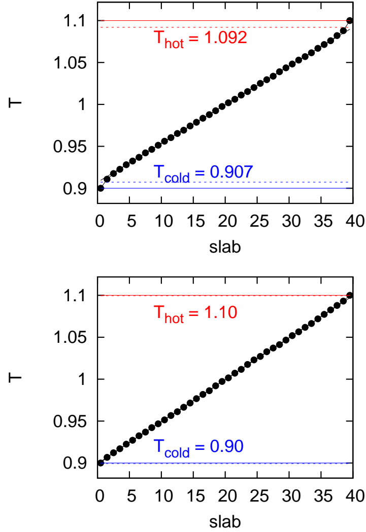
Figure 3.5: Temperature profile with a temperature gradient maintained by thermostats in front of two planar walls at the boundaries. Left side uses \alpha = 30^\circ and right side \alpha = 120^\circ . The collision time is h = 0.1 in both cases.
