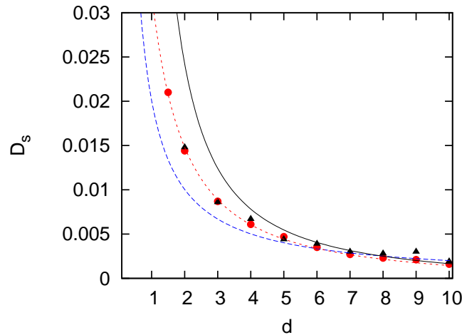
Figure 5.16: Self-diffusion coefficient vs. particle size for repulsive LJ colloid-solvent interactions. Symbols are simulation results, circles with fixed system size L = 30 , and triangles with fixed ratio \sigma/L = 1/12 . Lines correspond to the Einstein-relation in Eq. (5.14). The blue dashed line is the first term with Stokes friction (Eq. (1.23)) and the solid line corresponds to both terms in Eq. (5.14), including Enskog friction and the finite-size correction of the Stokes friction. The red dashed line is a fit to Eq. (5.14) with a colloid radius R + \Delta R , with \Delta R = 0.35 .
