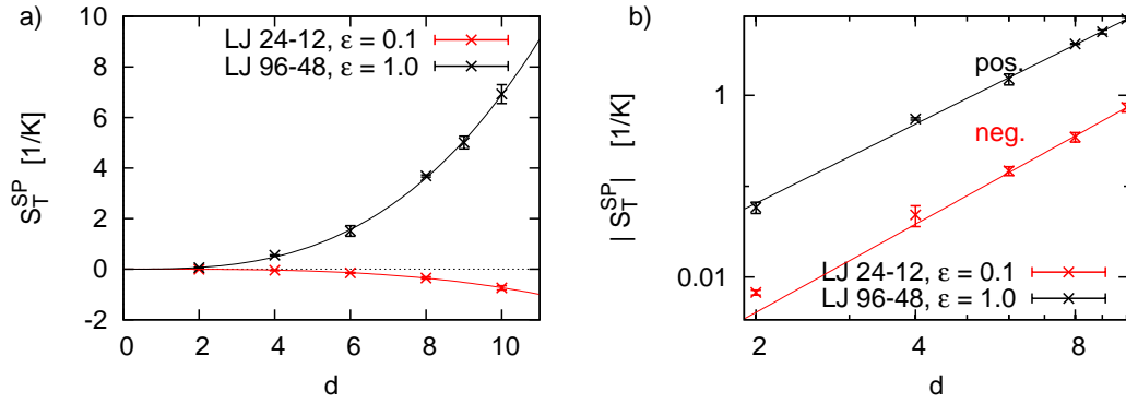
Figure 5.12: Dependence of the Soret coefficient on the particle size for different attractive Lennard-Jones potentials. The average temperature is T = 1.0 . Simulations with fixed \sigma_{cs}/L = 1/12 ratio. a) data with power laws fits b) double logarithmic plot, cubic power law dependence
