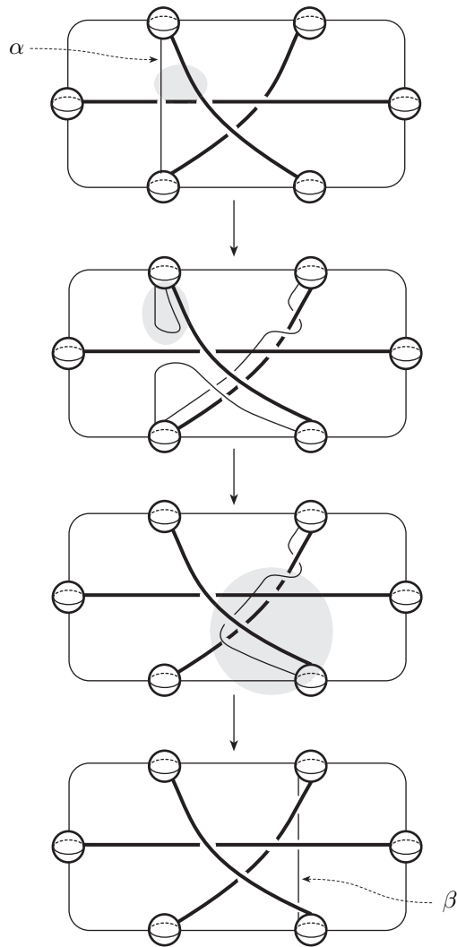
Figure A.4: Computation of the image of \alpha under \psi^{-1} . The shaded areas indicate that an isotopy or a handle slide is performed.
