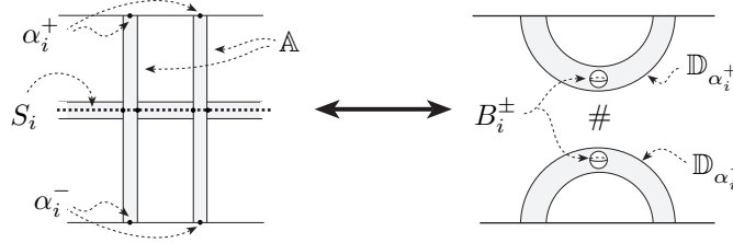
Figure 2.3: Relation between N(\gamma) and \#_g(H_0 \cup H_1) .
