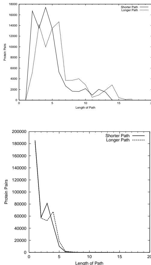
Fig. 6. Since G_d(\tau) is directed, and TP as well as FP are in the same SCC, directed paths going in both directions exist by definition. We show histograms of the shorter respectively longer path between false positives (top) and true positives (bottom). Observe the abundance of the latter for distance 3-5 and the existence of true positives at even larger distances up to a maximal distance of 13.
