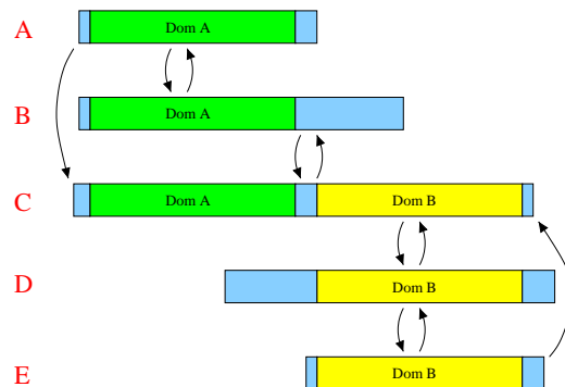
Fig. 9. This schematic picture shows a case where our simple heuristic fails. Due to the “ladder” of proteins with just the right increase in length, none of unwanted edges are removed when going over to the threshold graph. Such cases have been observed in the analysis of false positive appearing for lower thresholds \tau (not shown).
