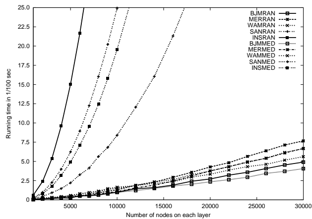
Fig. 6. Running time for sparse graphs
