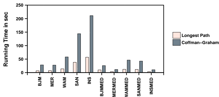
Fig. 9. Running time for AT&T graphs
