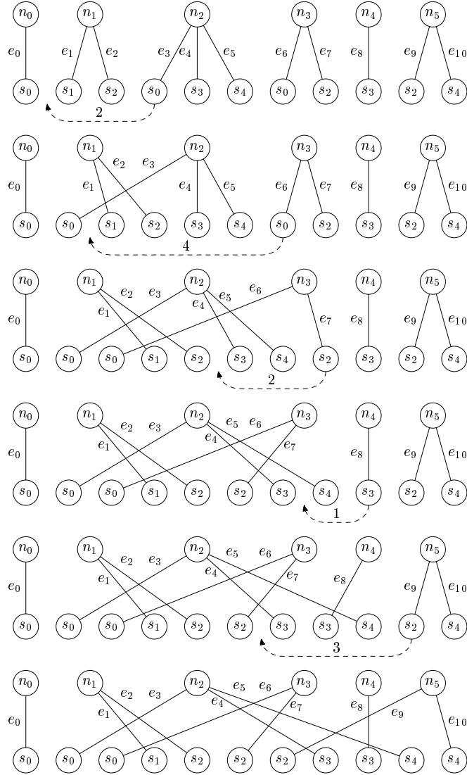
Fig. 3. Counting crossings via insertion sort
