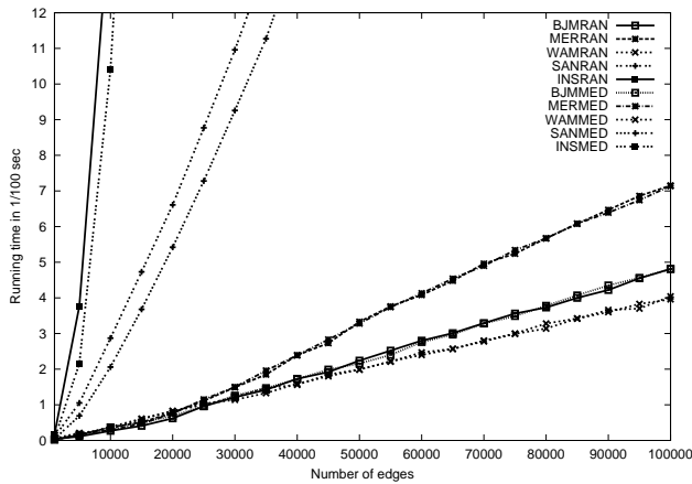
Fig. 8. Running time for graphs with increasing density
