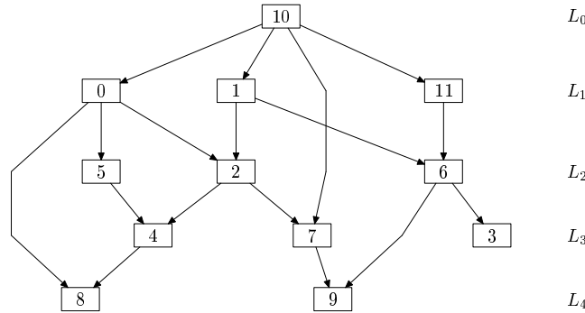
Fig. 2. A typical Sugiyama-style layout
