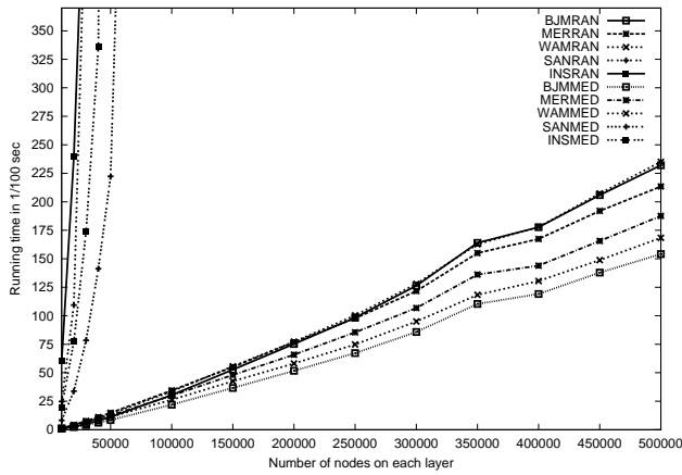
Fig. 7. Running time for large sparse graphs
