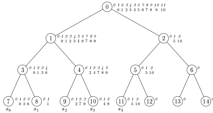
Fig. 4. Building the accumulator tree and counting the crossings
