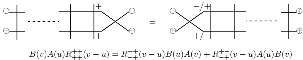
Figure 2.15.: A -operators
