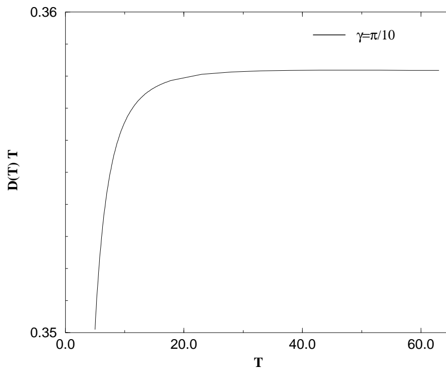
Figure 4.4.: The Drude weight at high temperature showing a 1/T -decrease ( \gamma = \frac{\pi}{10} ).
