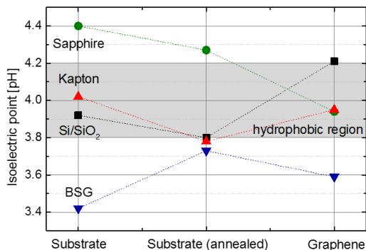
Figure 39: Comparison of IEPs for graphene layers on different substrates, original substrates and N_2 annealed substrates. Lines are guides for the eyes. The shaded regime represents the regime of IEP for hydrophobic materials.
