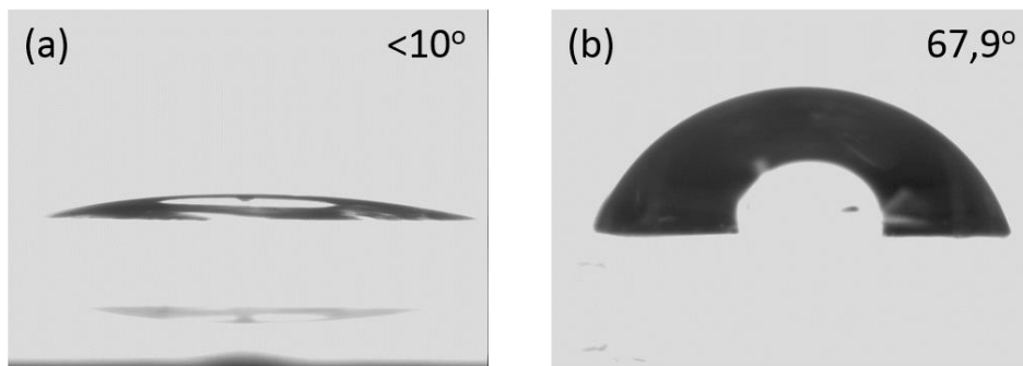
Figure 42: Contact angle measurements a) before and b) after the silanization of the borosilicate glass surface with APTES in the GLOBUS device.
