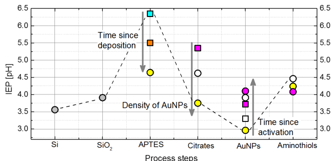
Figure 47: Resulting IEPs for the different process steps of immobilization and functionalization of gold nanoparticles, given in Figure 44. The dashed line shows the resulting modification of the \zeta potential. Different colors represent the different data sets.
