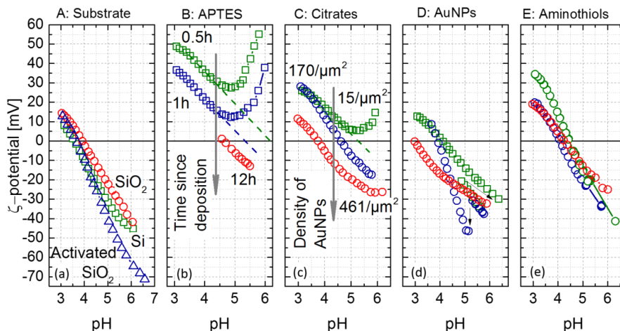
Figure 44: pH dependence of the \zeta potential of: (a) bare substrates Si, Si/SiO 2 and oxygen activated Si/SiO 2 , (b) after deposition of APTES (measured different time after APTES deposition), (c) after deposition of citrate-stabilized AuNPs (different AuNP concentrations are given), (d) after removal of free molecules (citrate and APTES) via oxygen plasma, and (e) after deposition of amino-1-undecanethiols onto the AuNPs. Each curve represents a different pair of samples, however, experiments in the same symbol (and color) belong to one series of measurements (e.g. identical density of AuNPs), and excluding step A, which is the same for all. Additional lines in (b) and (c) indicate the extrapolation of the measurement that is used to obtain an IEP value for some of the measurements.
