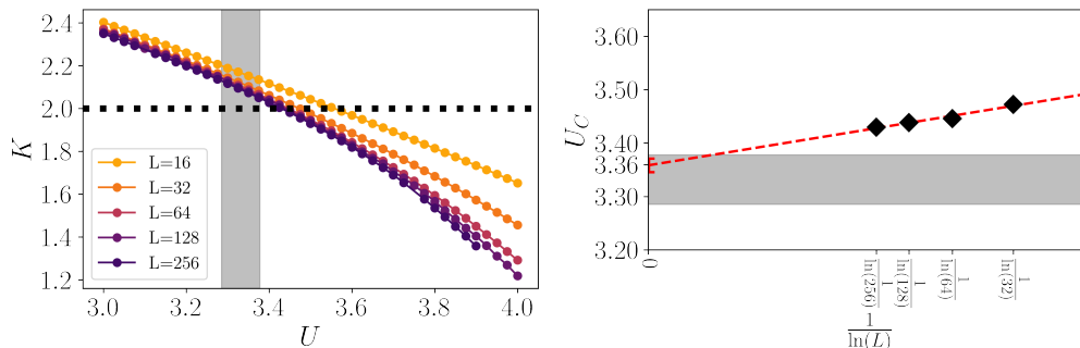
Figure A1: Detection of the BKT transition by means of the second moment of the PDF distribution, i.e. the number fluctuations (see [124]). ( left ) the curves of the effective Luttinger parameter K^* values for different sizes of the system as a function of U ( t = 1 and V = 0 ). The critical true value is expected at K = 2 from the Luttinger theory (dotted black line). The gray regions stand for the single standard deviation confidence interval as from the estimates of literature summarized in Table 1 of [107]. ( right ) shows with diamonds the pseudo-critical values extracted from the crossing of the K^* curves with K = 2 , as a function of the reciprocal of the log-size. With a linear fit (red dashed line) the extrapolation of U_C to the thermodynamic limit is the intercept.
