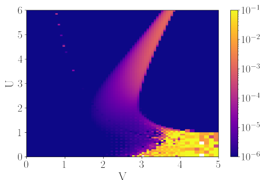
Figure 7.7: Phase diagram of the EBH model drawn with the residuals of the PDF's fit including the linear term for a L = 64 system. The SS+SF and HI regions are identified by the high value of the residuals.
