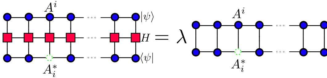
Figure 2.10: Pictorial representation of the step of the variational iterative ground-state search.
