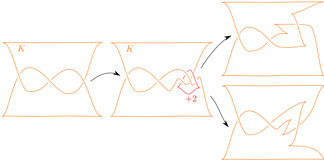
Figure 7.6: A surgery description of a Legendrian trefoil
