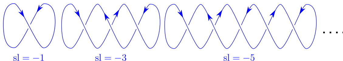
Figure 2.17: A complete list of transverse unknots
