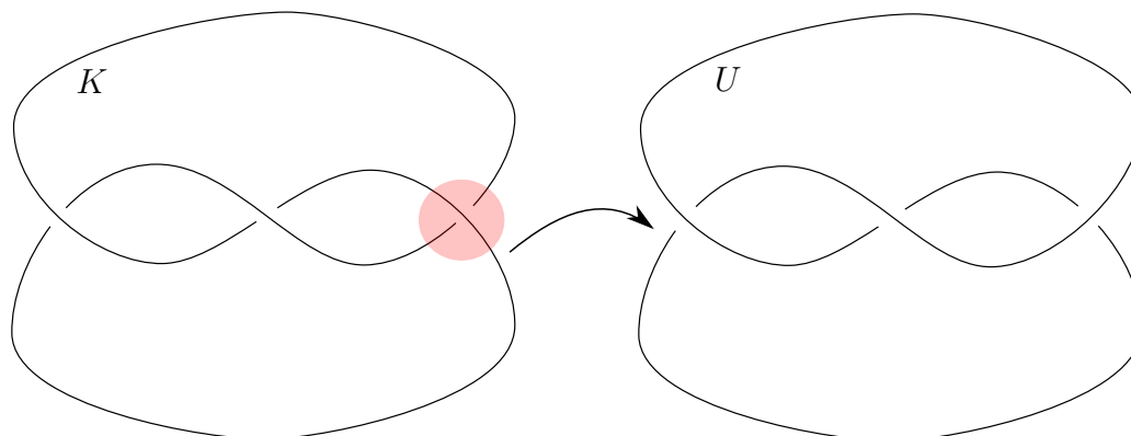
Figure 7.1: Transforming the trefoil knot to the unknot by changing a crossing again S^3 , but the type of the marked crossing changes. So this surgery changes the knot type of K to the unknot in S^3 .
