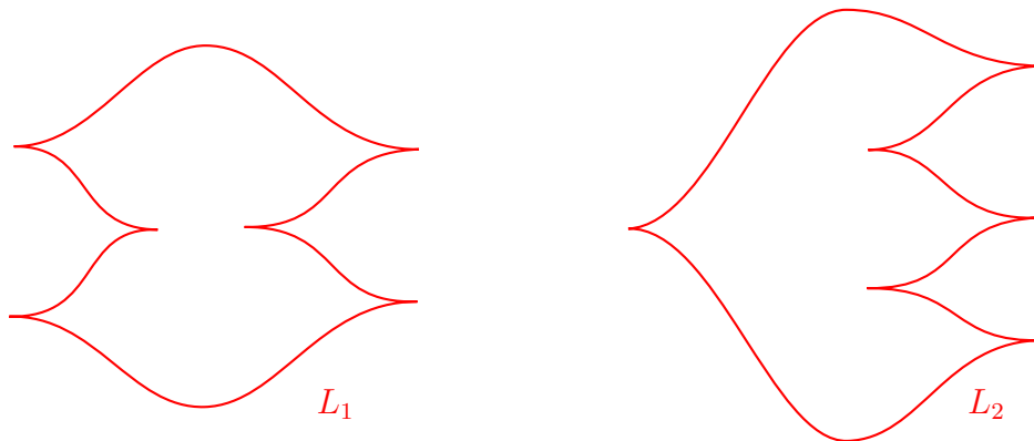
Figure 2.14: Different Legendrian unknots with same tb invariants
