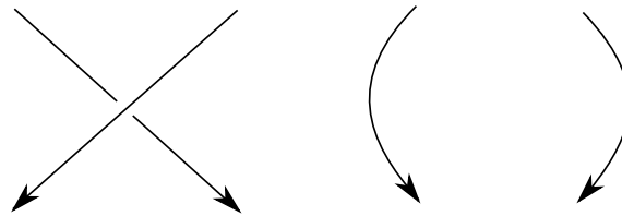
Figure 2.5: Impossible front projections of positive transverse knots
