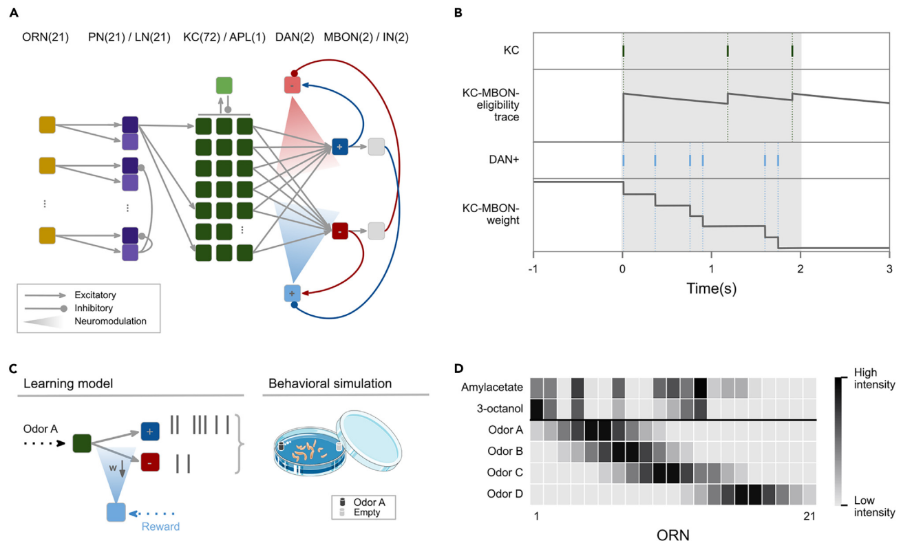
Figure 1. Network mechanisms
