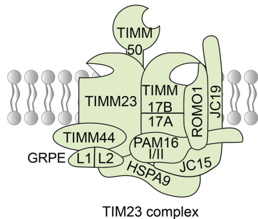
Figure 6. Structure of the human TIM23 complex. The TIM23 complex, embedded in the IM, consists of two half-channels formed by TIMM23 and TIMM17 homologs, with TIMM17 functioning as the translocation pore. This pore is shielded by ROMO1 to facilitate protein import into the mitochondrial matrix and by acting as a gate, enabling the insertion of proteins into the IM. The PAM complex, essential for ATP-driven translocation, comprises TIMM44, GRPE homologs, HSPA9, which mediates ATP hydrolysis, as well as PAM16 and J-domain protein homologs.
