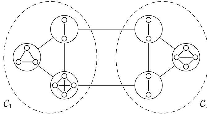
Figure 4.3: An equidominating graph consisting of the two clique bundles \mathcal{C}_1 and \mathcal{C}_2 each containing three clique classes with two to four vertices; clique classes are indicated by circles and an edge between the circles of two clique classes represents all edges between the vertices of the corresponding clique classes.
