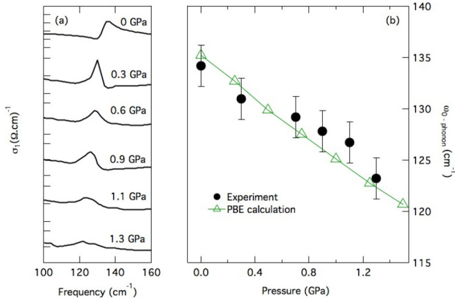
FIG. 3. (a) Detail of the B_{1u} phonon mode for selected pressures. (b) Pressure-dependent B_{1u} phonon frequency from experimental data and ab initio calculations described in Sec. V.
