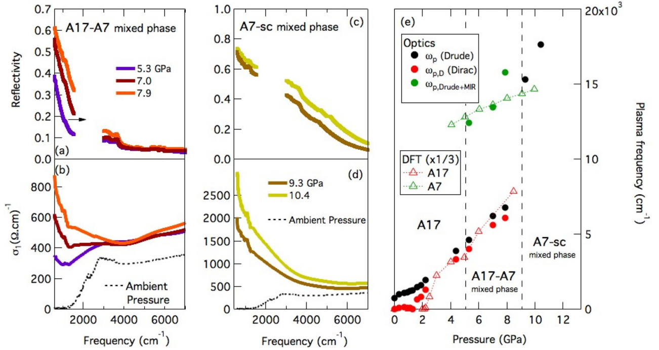
FIG. 4. Optical reflectivity at the sample-diamond interface (a) and real optical conductivity (b) of BP measured along the c -axis polarization direction in the A17-A7 mixed phase. (c)-(d) Same quantities in the A7-sc mixed phase. The ambient pressure optical conductivity is reported for comparison as a dashed line in panels (b) and (d). (e) Experimental (full circles) and theoretical (empty triangles) Drude plasma frequencies across the structural phase transitions. Black circles represent the bare Drude-Lorentz plasma frequency. The Dirac plasma frequency (red circles) is obtained by subtracting the plasma frequency of the thermally activated massive carriers. The sum in quadrature of the Drude and MIR band plasma frequencies is shown as green circles. Red and green triangles are the rescaled DFT plasma frequencies in the A17 and A7 phases, respectively.
