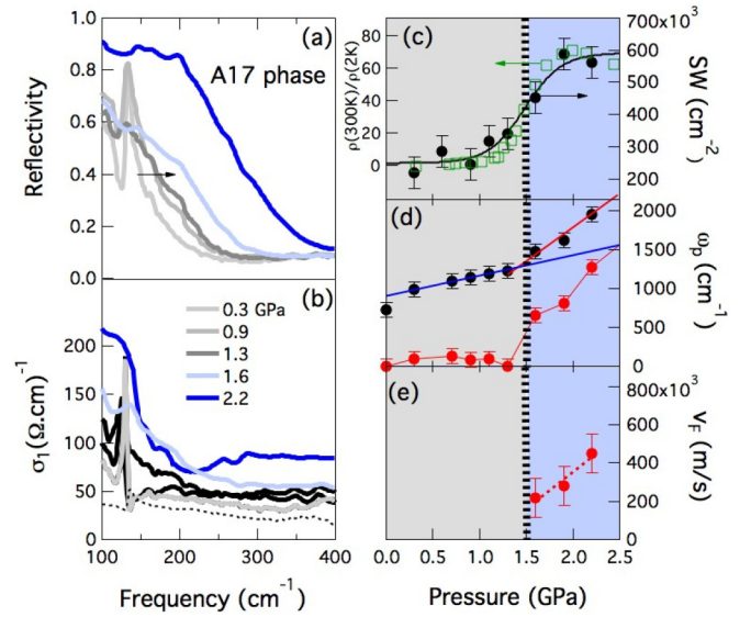
FIG. 2. Optical reflectivity at the sample-diamond interface (a) and real part of the optical conductivity (b) of orthorhombic BP measured along the c -axis polarization direction. The ambient pressure optical conductivity is also reported for comparison as a black dashed line. (c) Spectral weight (SW) of \sigma_1(\omega) integrated between 100 and 200 \text{ cm}^{-1} . SW follows a phenomenological sigmoid behavior centered at P_L = 1.5 \text{ GPa} (dashed vertical line). The resistivity ratio \rho(300 \text{ K})/\rho(2 \text{ K}) from Ref. [9] is also reported for comparison. (d) Plasma frequency \omega_p (from Lorentz-Drude fitting) vs pressure. Black circles represent the bare \omega_p , while red circles mark the Dirac \omega_p (see text). (e) Fermi velocity of Dirac carriers from Eq. (1). The red dashed line is a guide to the eye.
